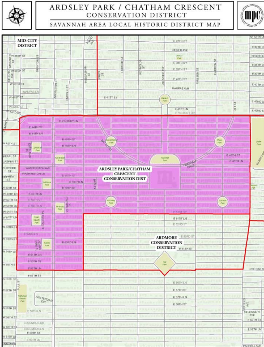
Map 1: Ardsley Park-Chatham Crescent Conservation District (CD-1)
